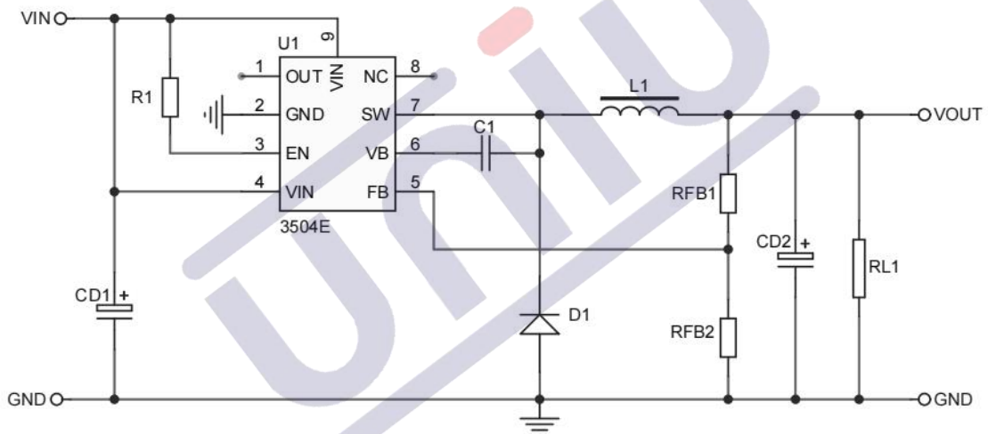
APP2: V_{OUT}<10V
