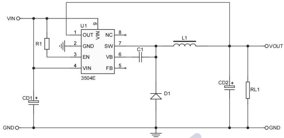
APP2: V_{OUT}<10V
