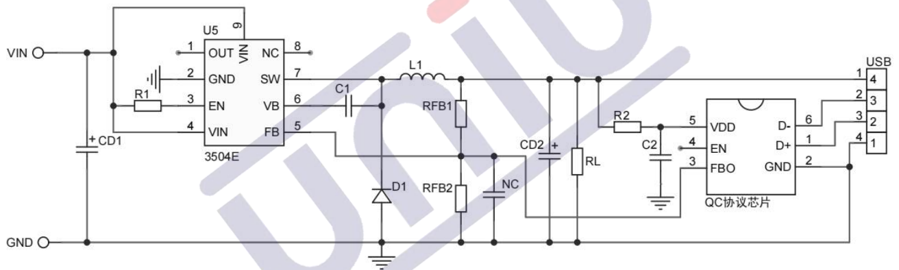
APP5:QC2.0/QC3.0
